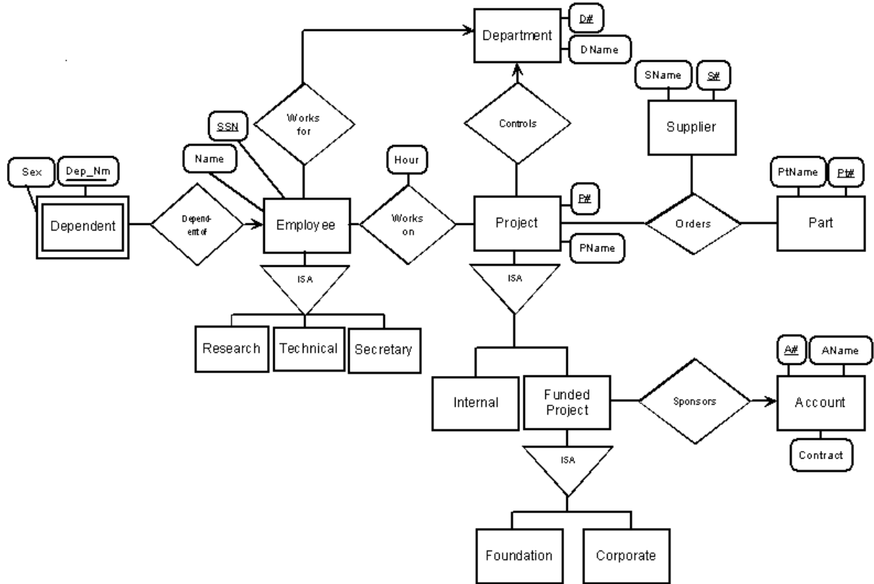
FIGURE 7: KORTH's Notation
