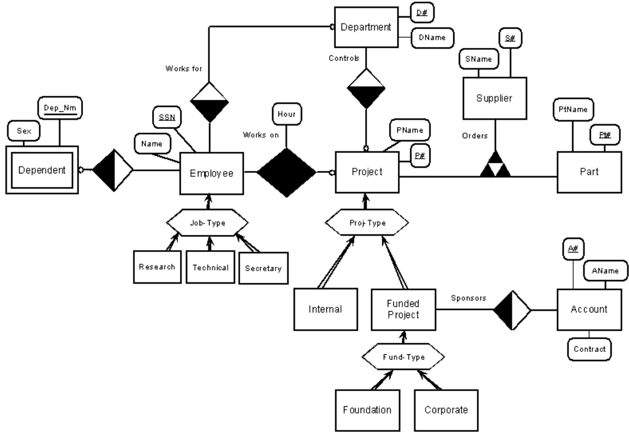
FIGURE 5: TEOREY's Notation
