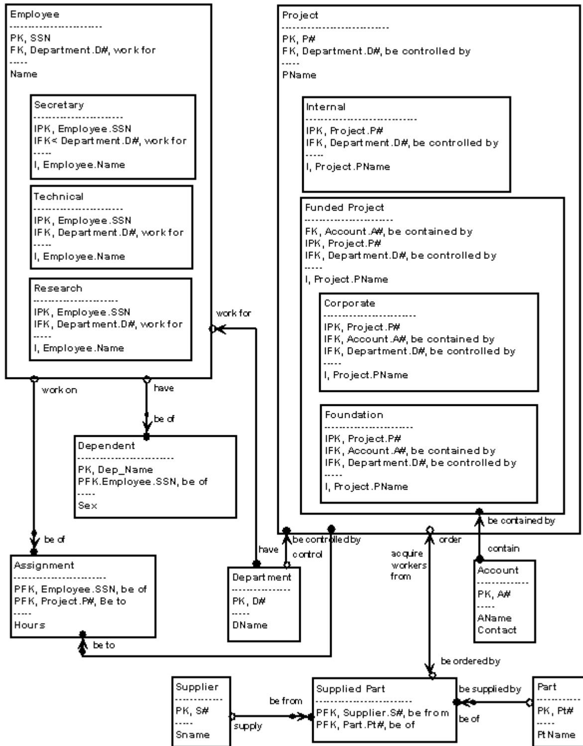
FIGURE 13: BACHMAN Notation
